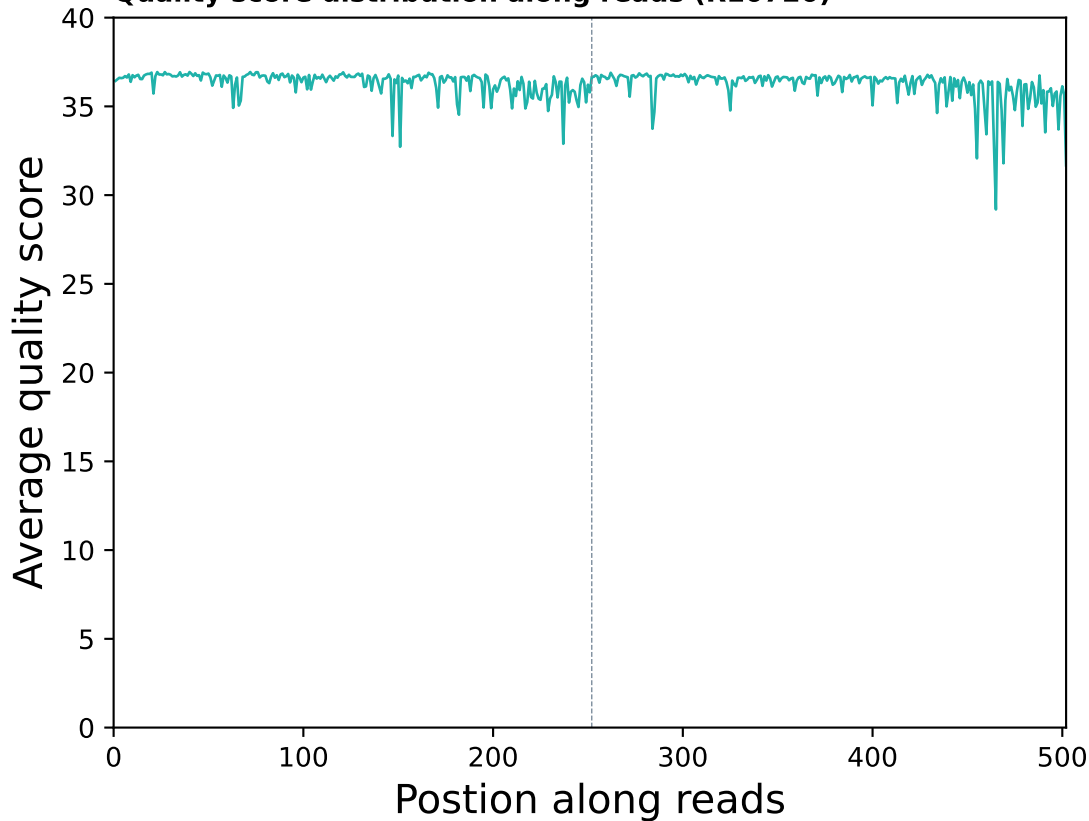
Quality score distribution along reads (R10720)
